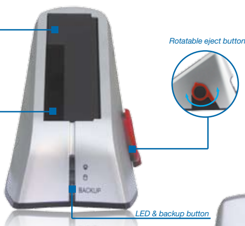
Slot for 3.5" SATA HDD
